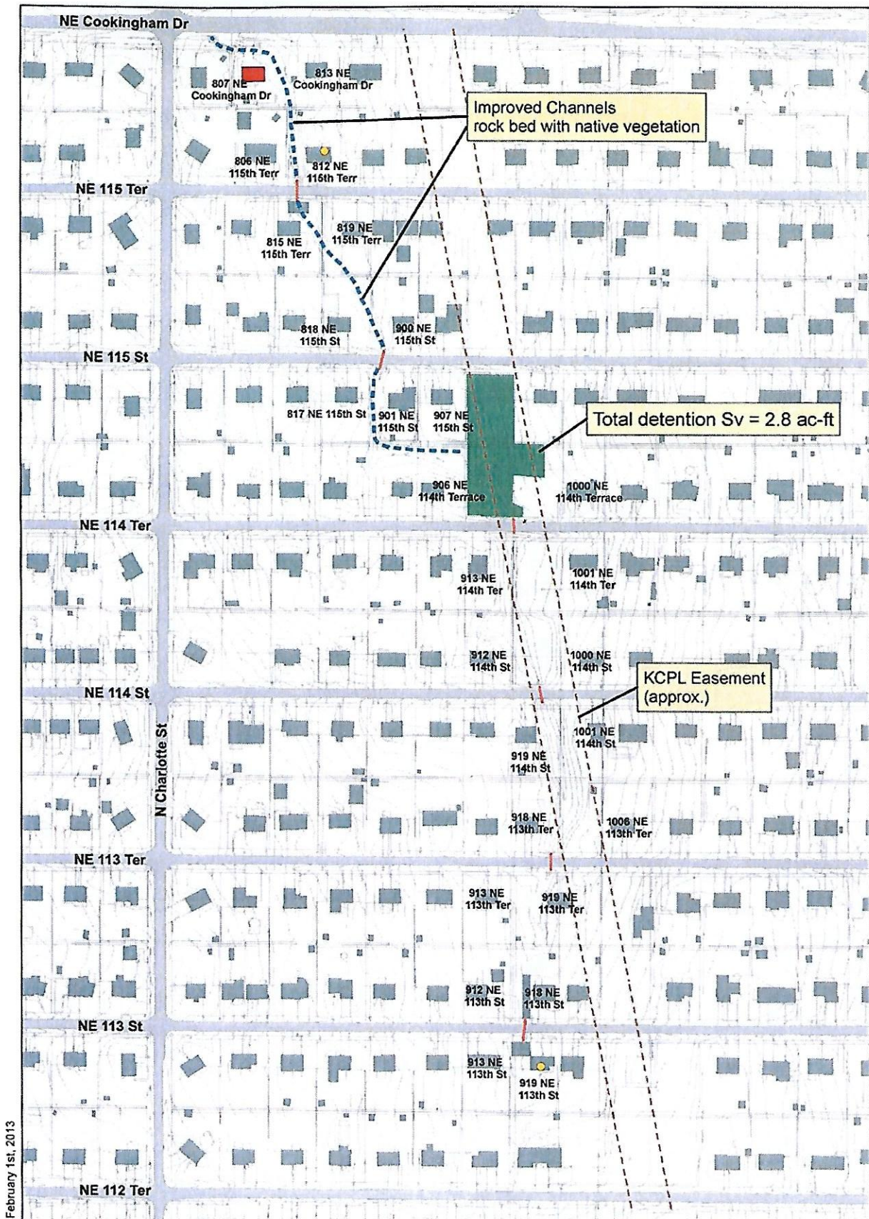
Figure 3 - Option 1 NE Cookingham Stormwater Improvements Kansas City, MO
